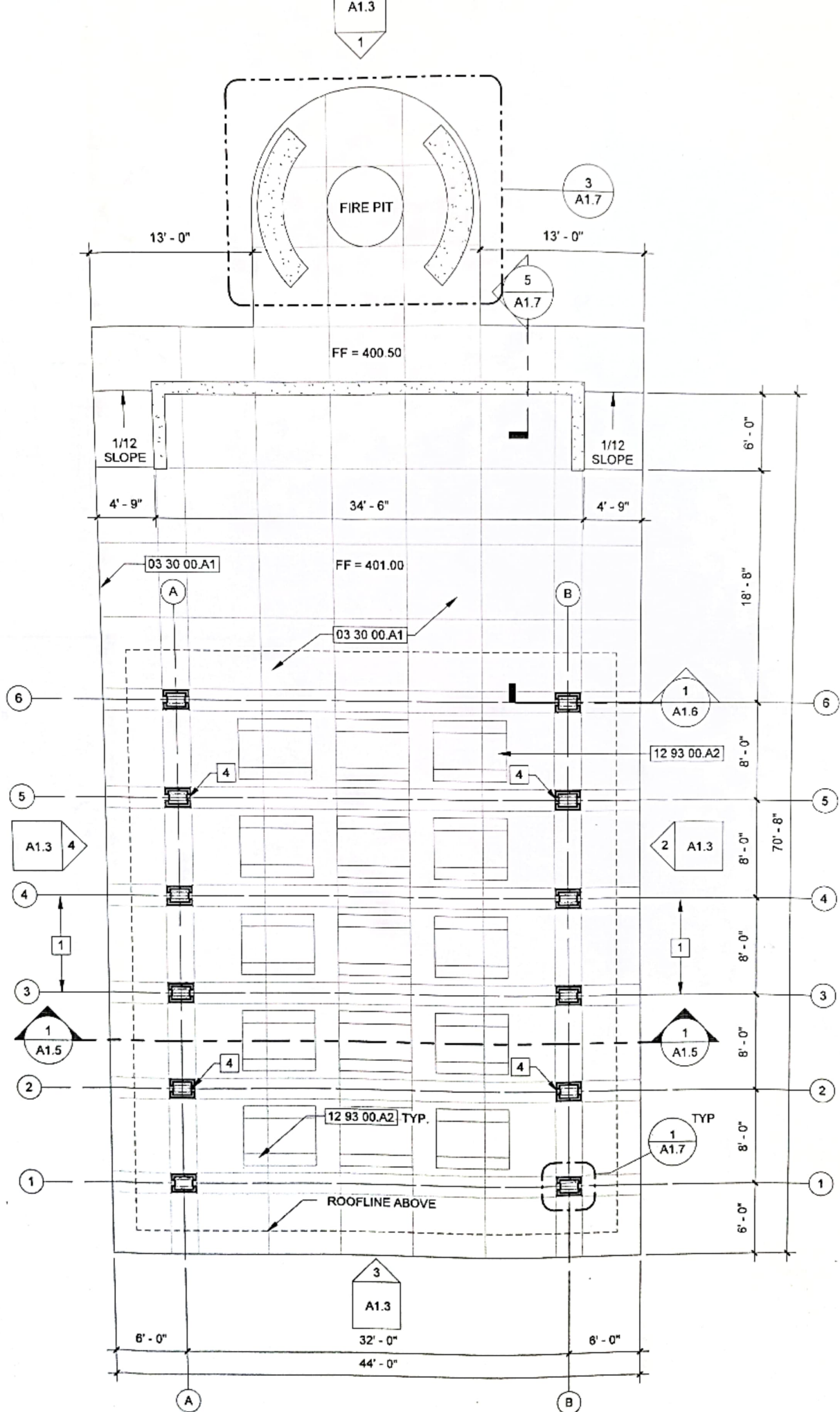
1 EAST PAVILION FLOOR PLAN 1/8" = 1'-0"
